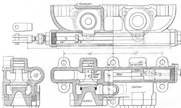
Figs. 2227-2230, By-Pass and Starting Valve for Schenectady Tandem Compound Locomotive. American Loco. Co.
